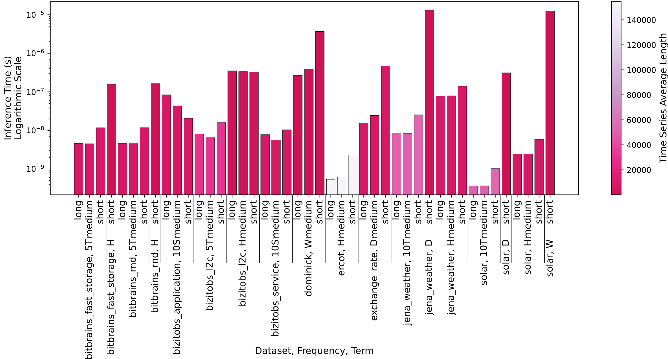
Normalized Inference Time per Dataset - Model: TimesFM-1.0
