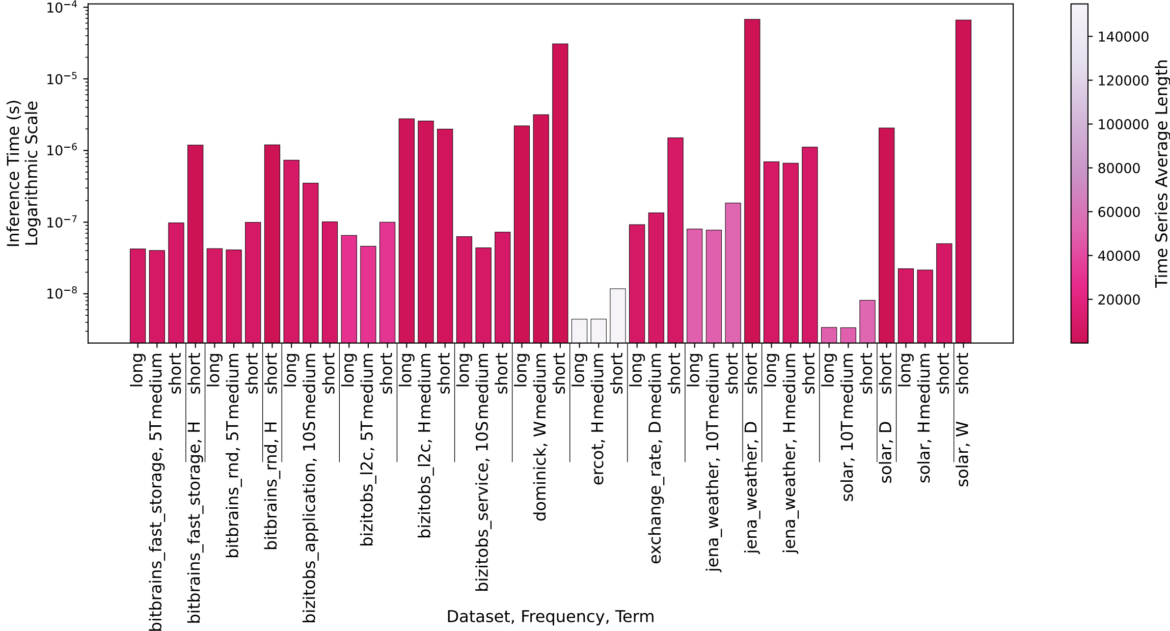
Normalized Inference Time per Dataset - Model: TimesFM-2.0
