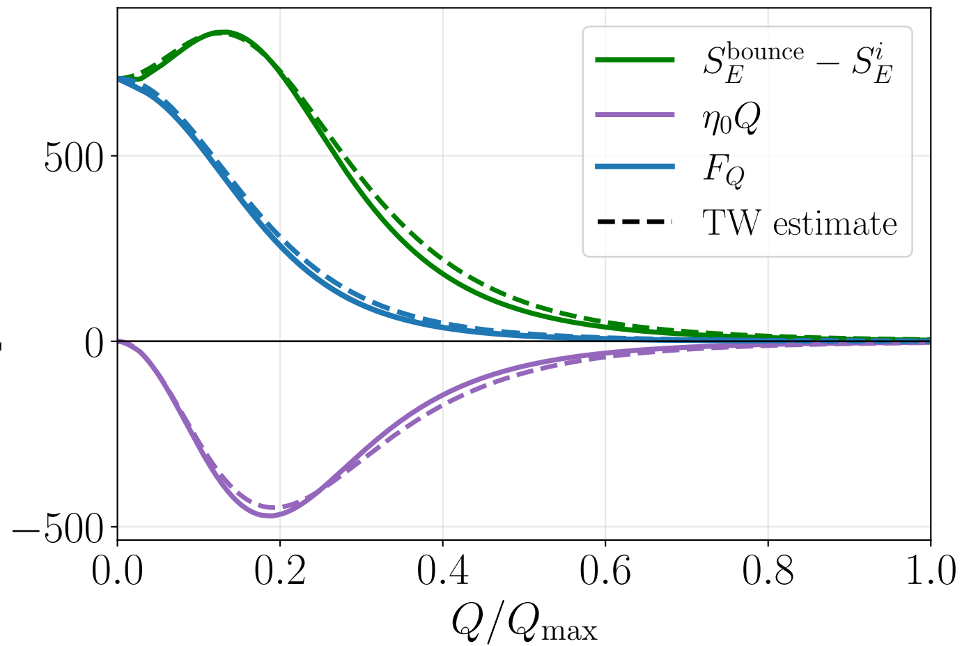
Thin wall: \rho_0 = 2 - 10^{-9}
