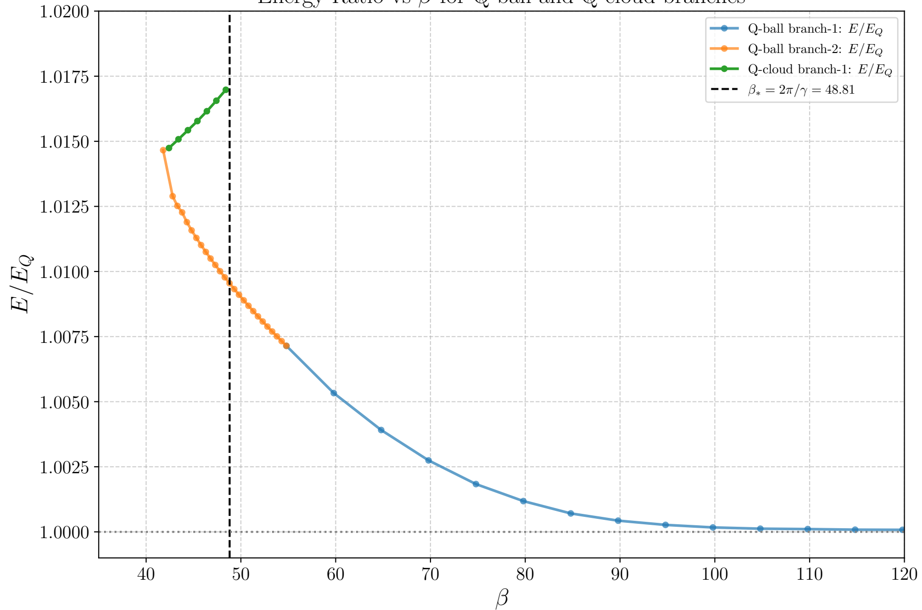
Energy Ratio vs \beta for Q-ball and Q-cloud branches
