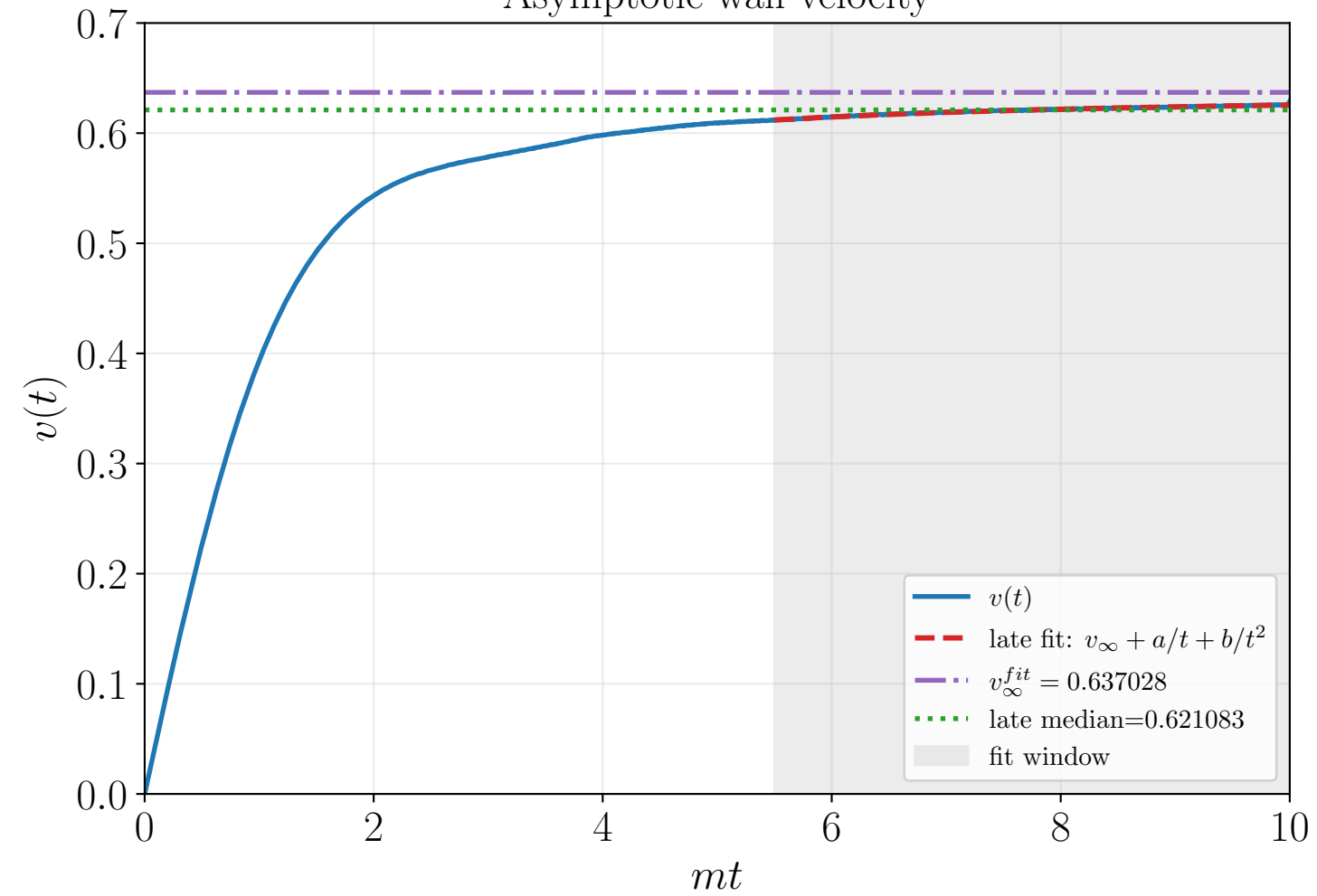
Asymptotic wall-velocity
