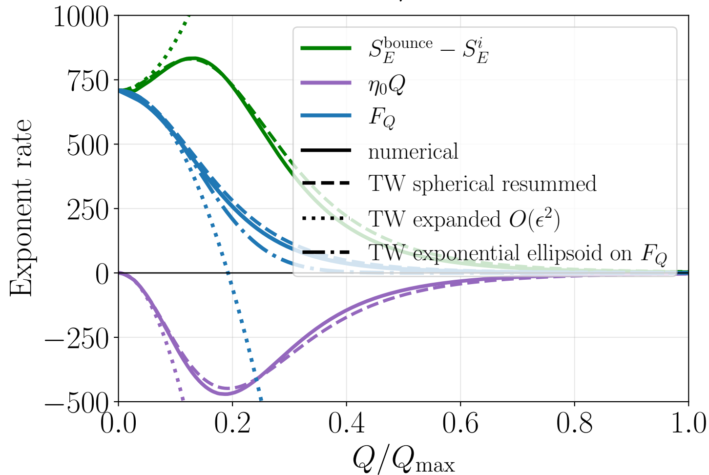
Thin wall: \rho_0 = 2 - 10^{-9}
