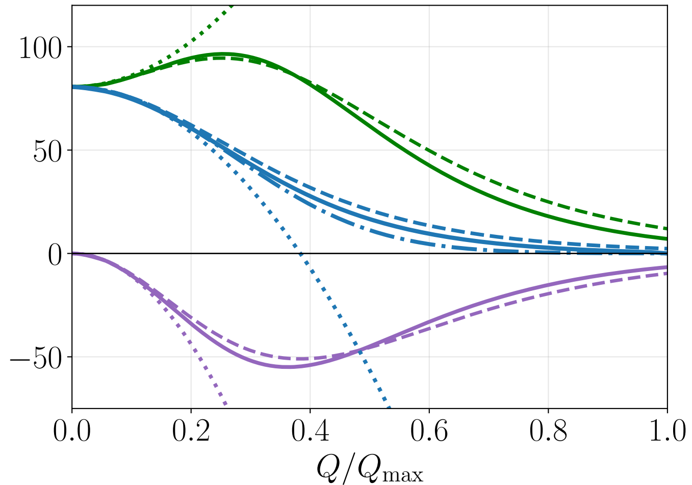
Thick wall: \rho_0 = 2 - 10^{-3}
