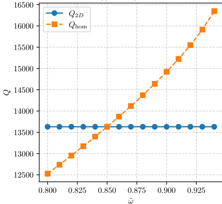
(i) Charge vs \omega
