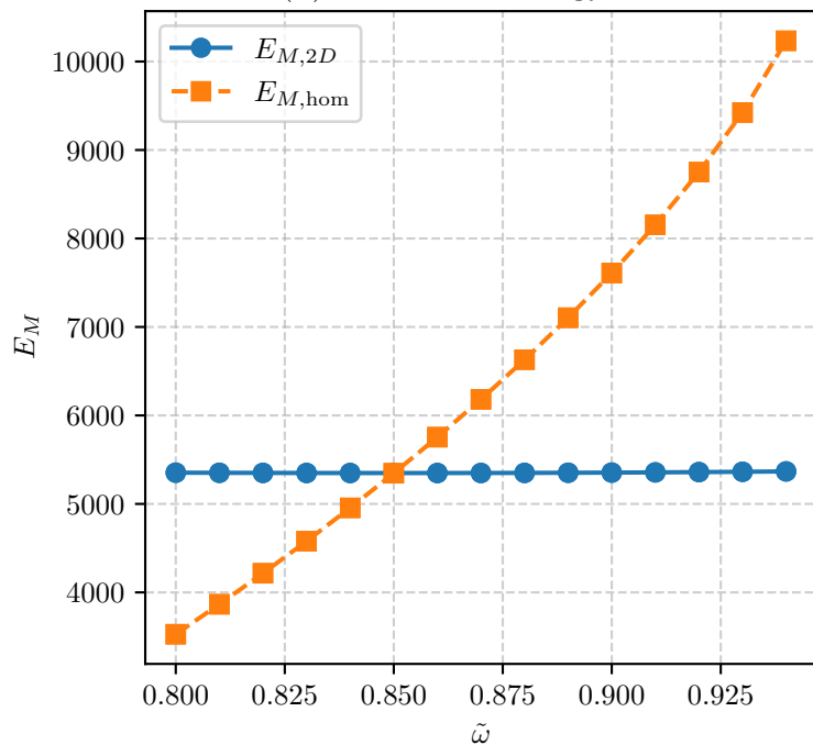
(ii) Minkowski energy vs \omega
