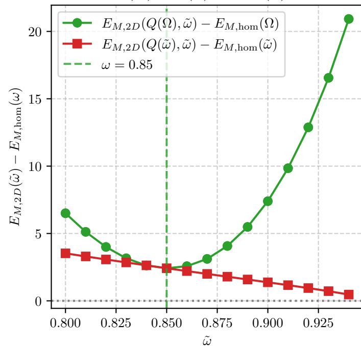
(iii) E_{2D}(\tilde{\omega}) - E_{\text{hom}}(\omega)
