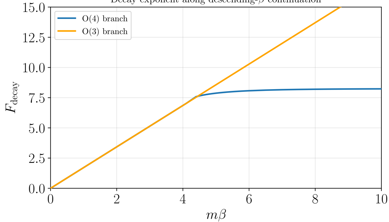
Decay exponent along descending- \beta continuation
