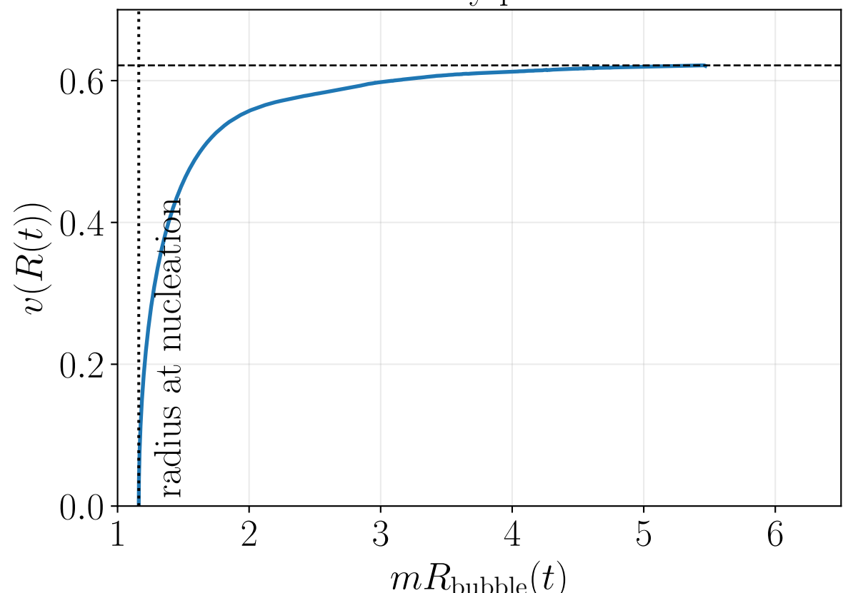
Velocity profile
