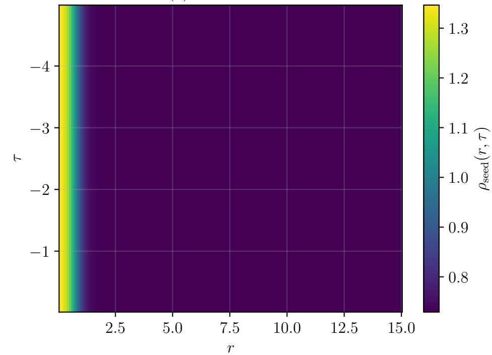
O(3) static: 2D seed
