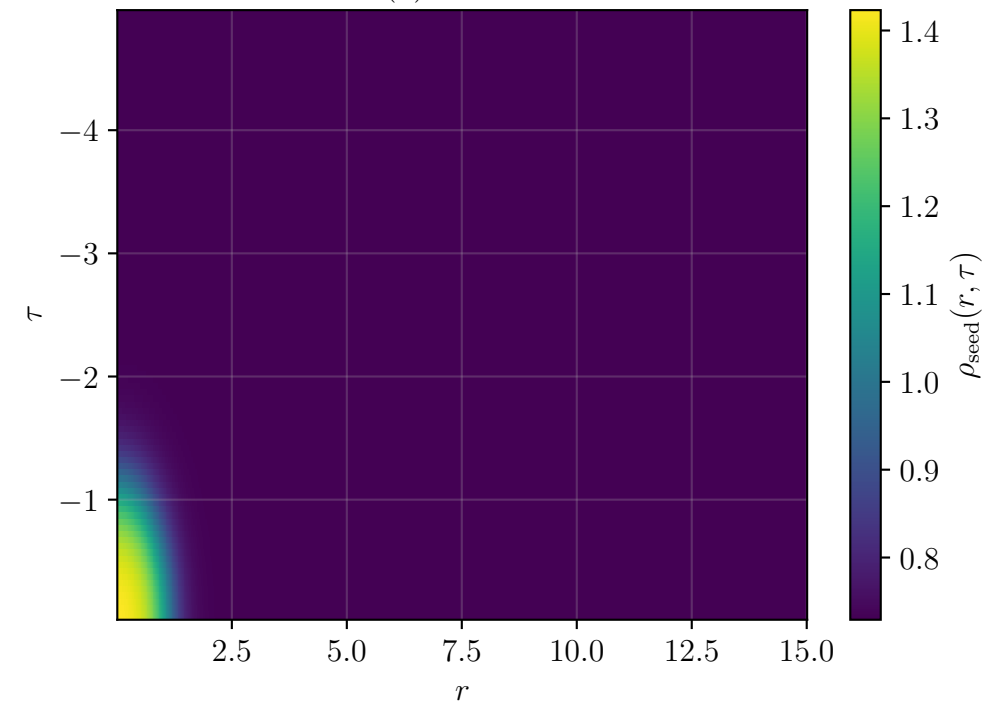
O(4): 2D seed
