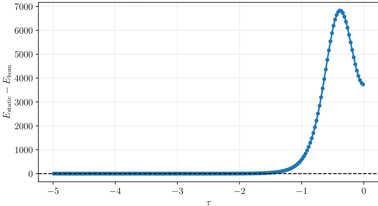
O(1) r -static: static energy diagnostic
