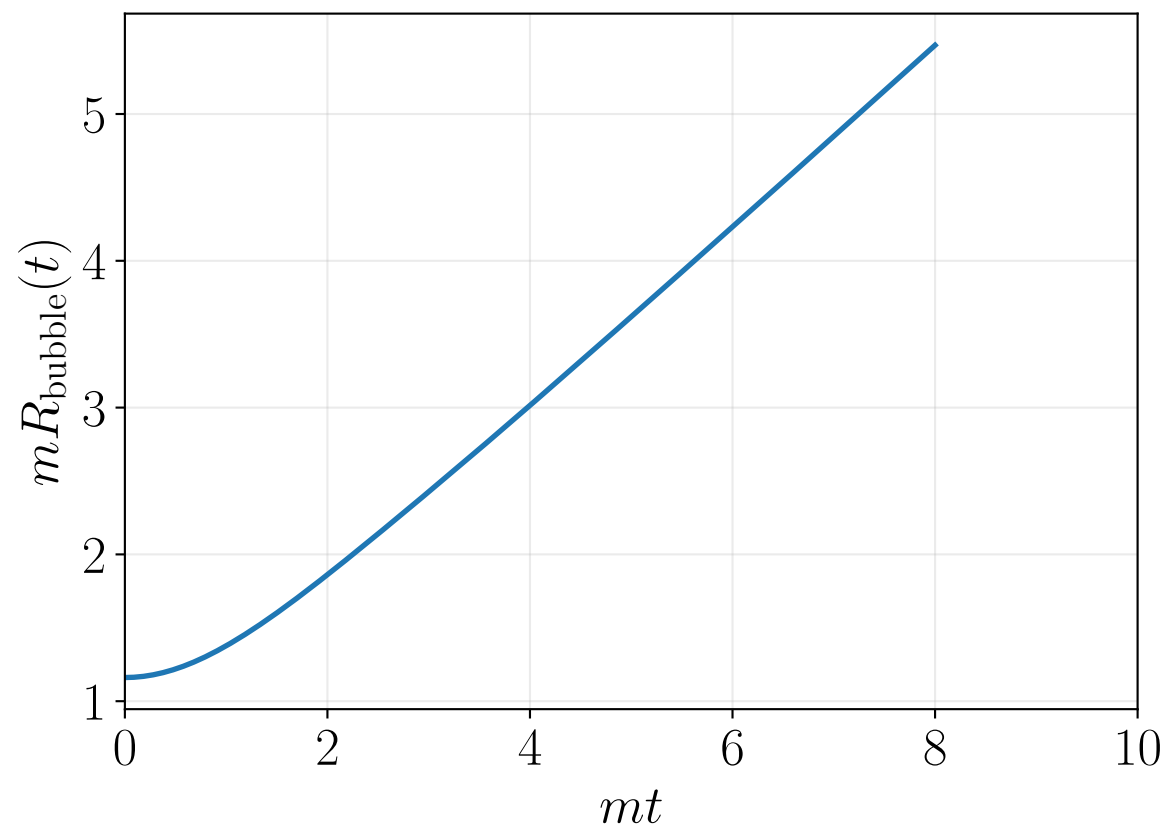
Bubble radius evolution
