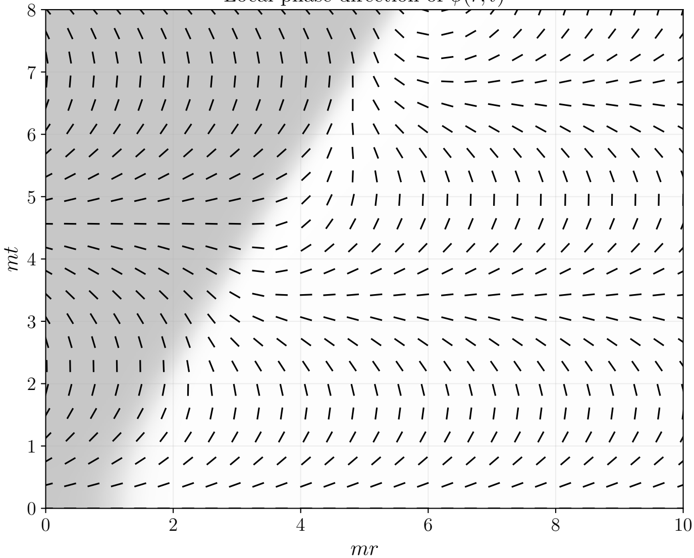
Local phase direction of \phi(r, t)
