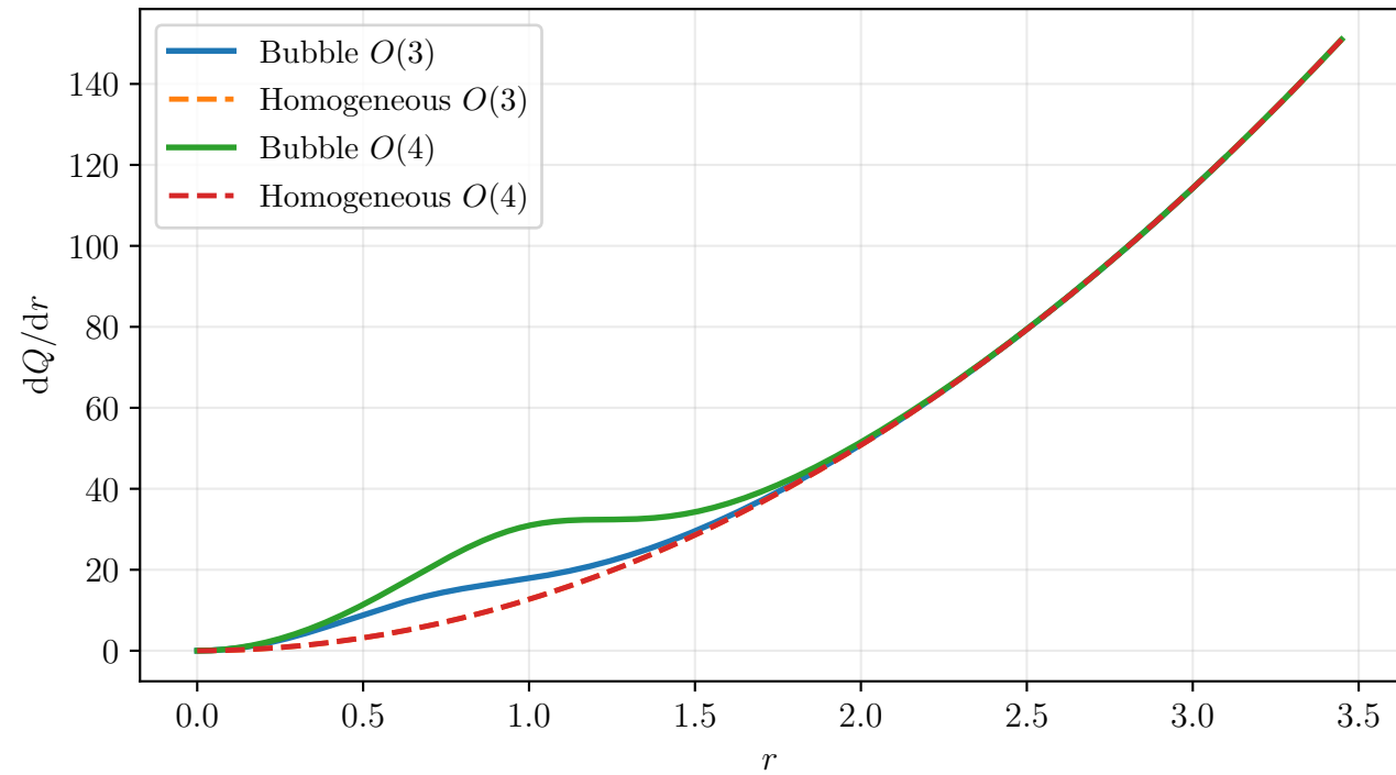
Radial charge integrand
