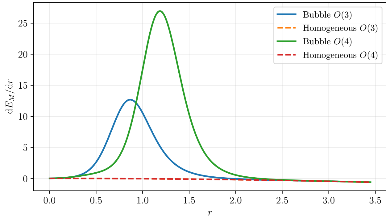
Radial Minkowski-energy integrand
