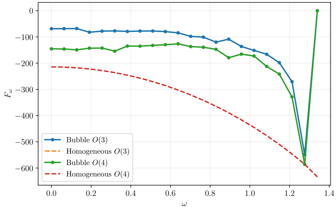
F_\omega vs \omega at fixed V_{\text{ref}}
