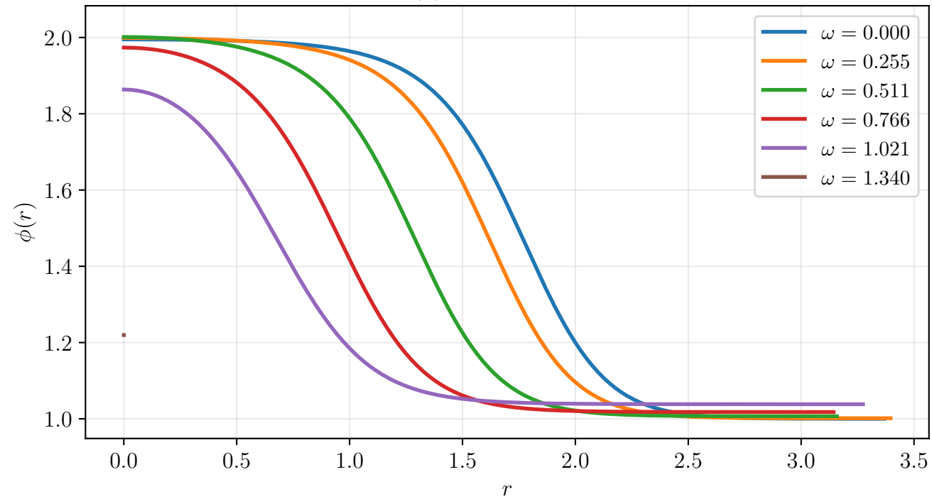
O(3) profile evolution
