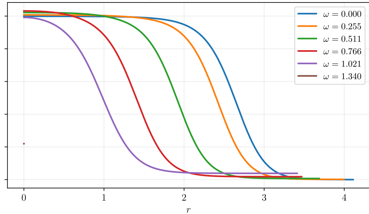
O(4) profile evolution
