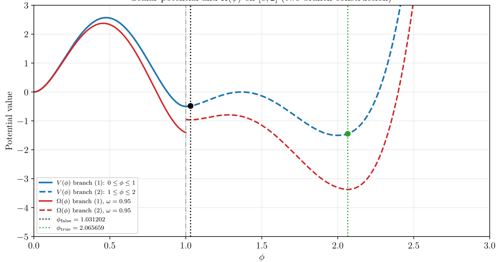
Scalar potential and \Omega(\phi) on [0, 2] (two-branch construction)
