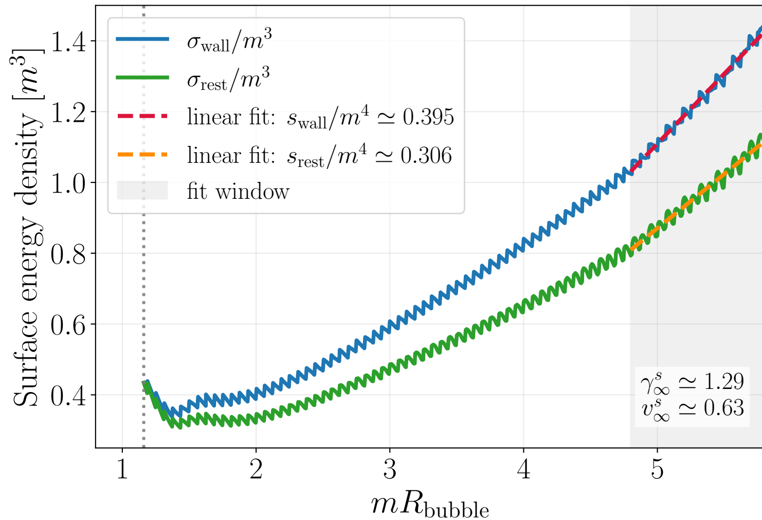
Wall tension vs radius
