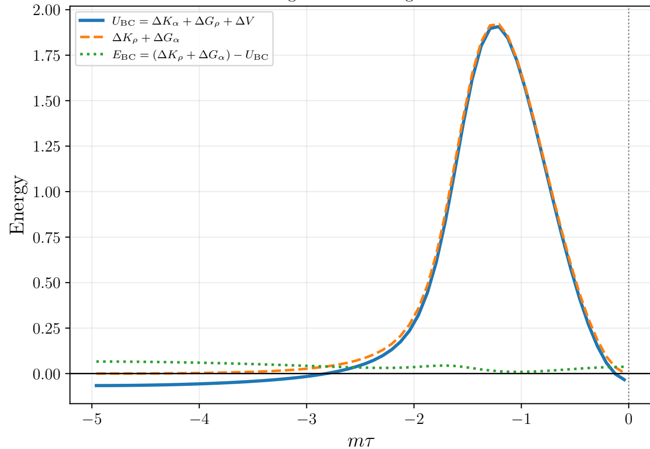
Charged Bitar–Chang barrier
