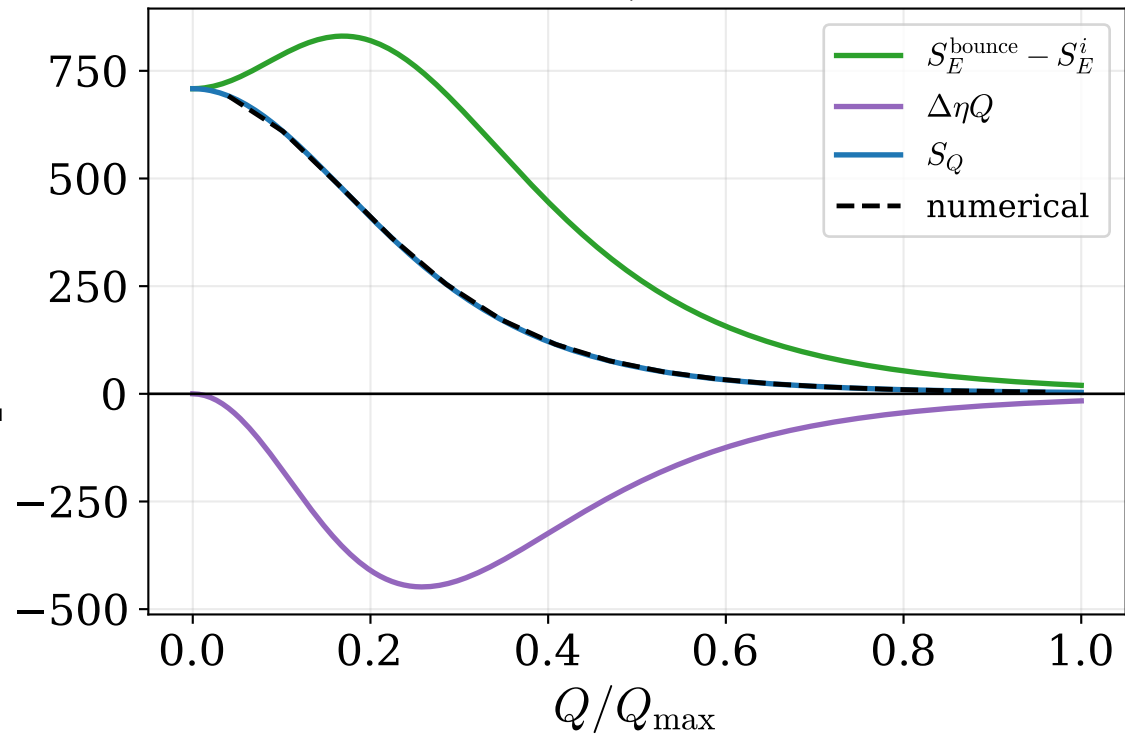
Thin wall: \rho_0 = 2 - 10^{-9}
