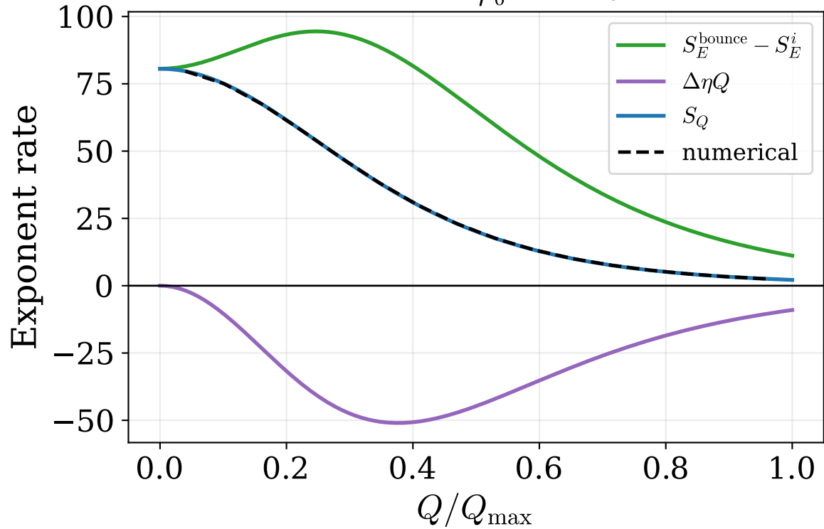
Thick wall: \rho_0 = 2 - 10^{-3}
