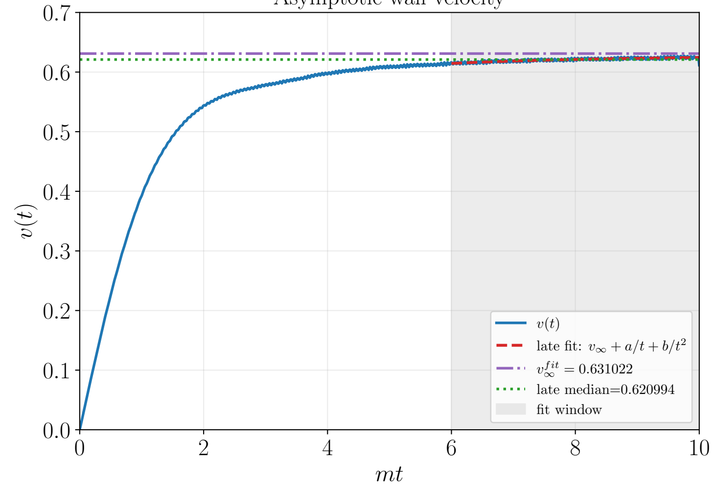
Asymptotic wall-velocity
