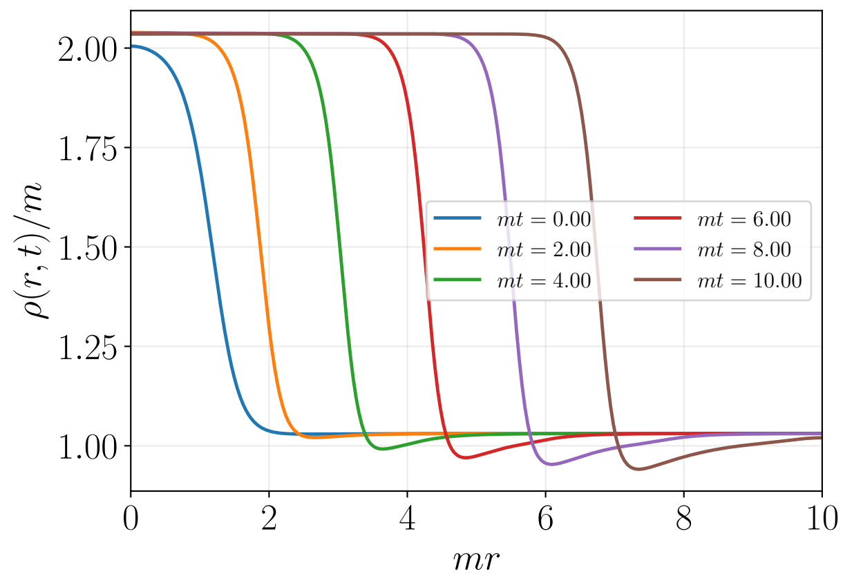
Bubble radius evolution
