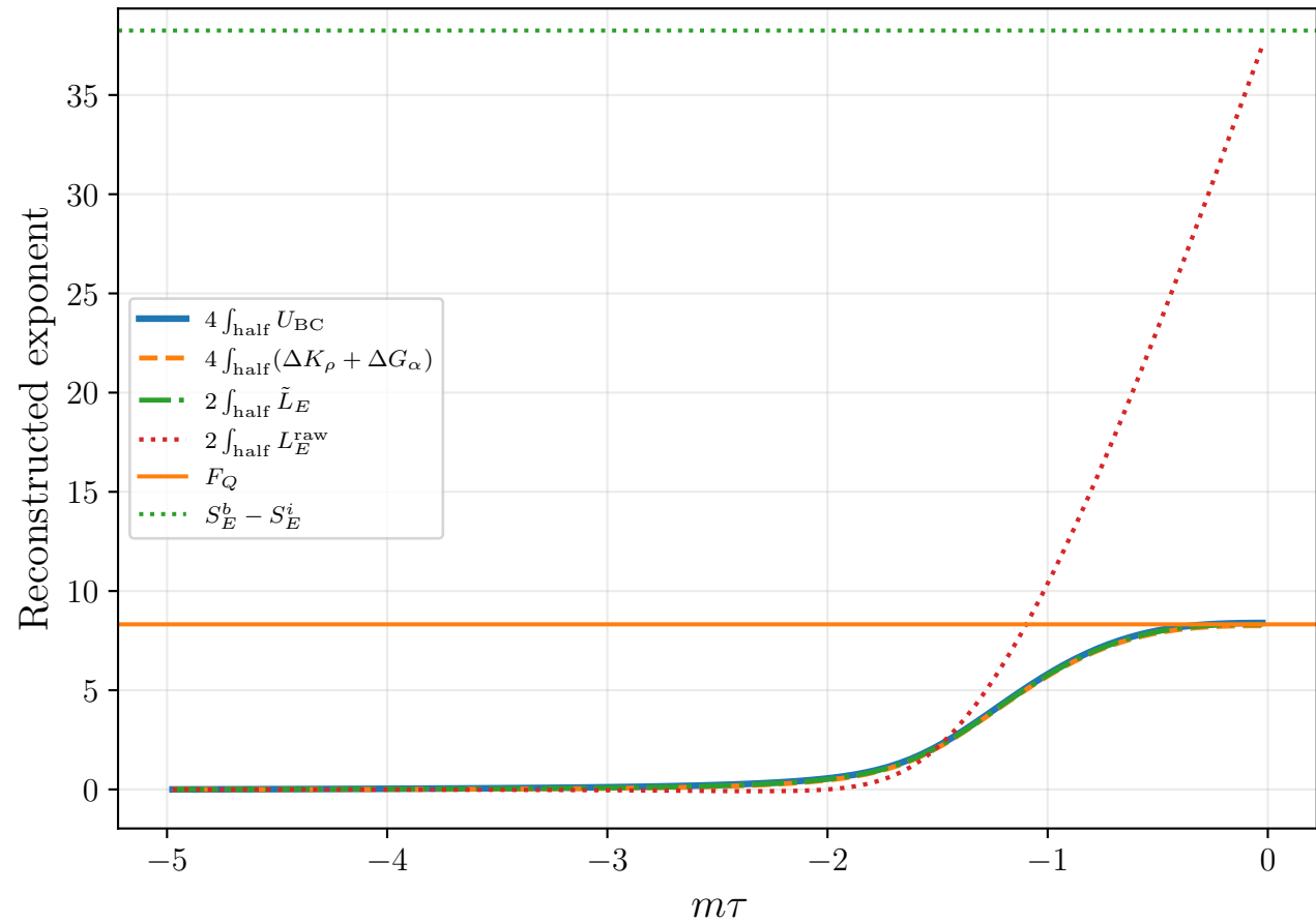
Cumulative reconstruction
