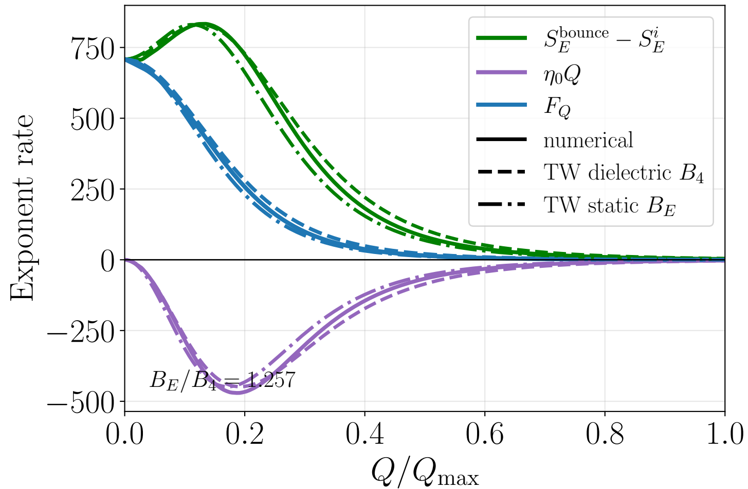
Thin wall: \rho_0 = 2 - 10^{-9}
