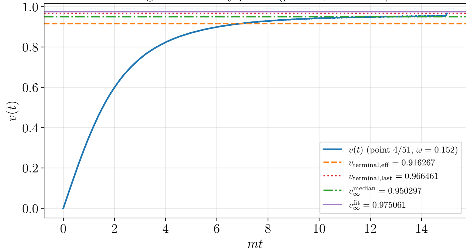
Omega-scan velocity profile (point 4, \omega = 0.152 )
