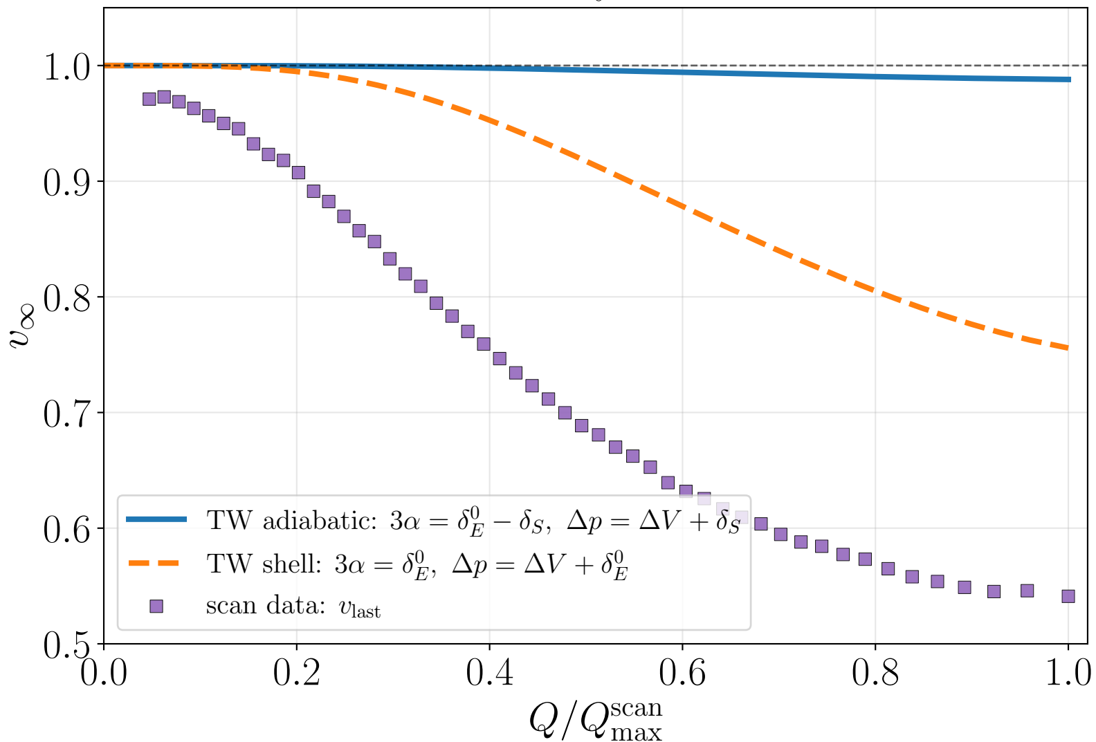
TW terminal velocity estimates at \tau = 0
