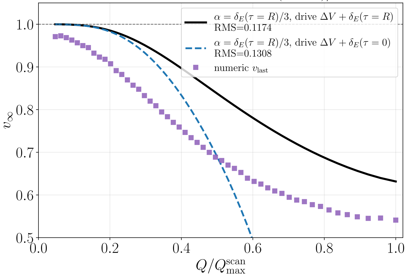
TW estimate for v_\infty : \alpha = \delta_E(\tau = R)/3
