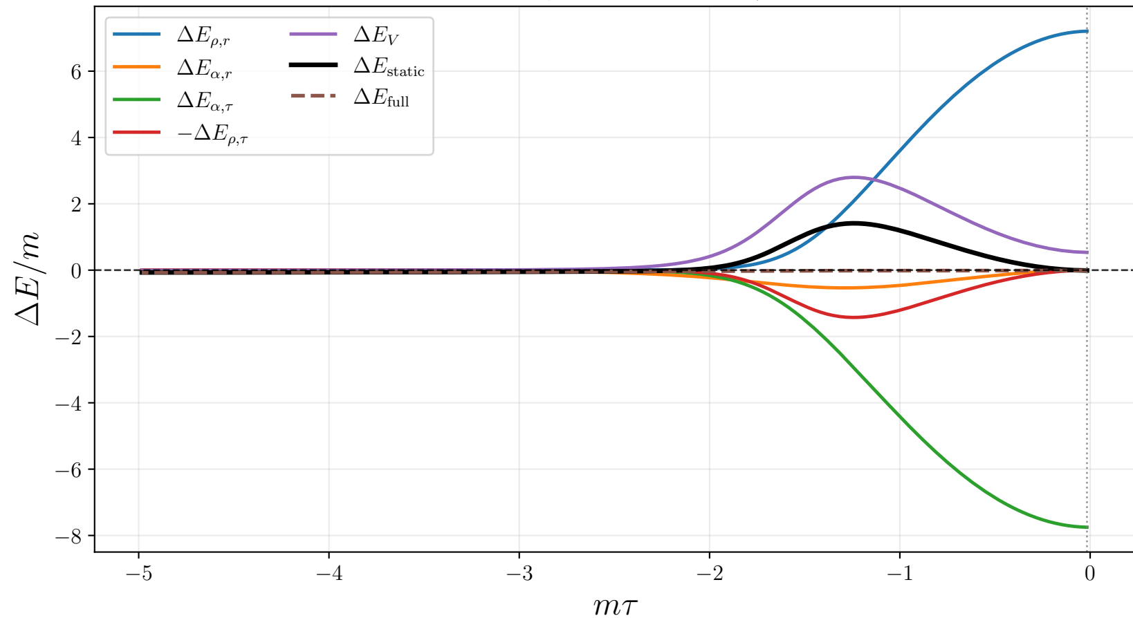
Euclidean energy decomposition in \rho and \alpha
