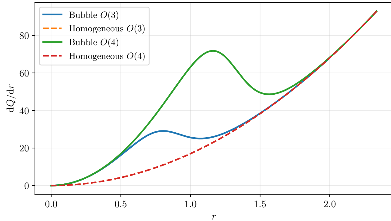
Radial charge integrand
