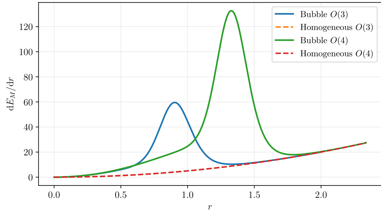
Radial Minkowski-energy integrand
