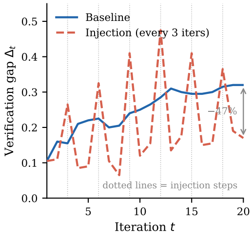
(b) Hard-negative injection reduces gap by 47\%
