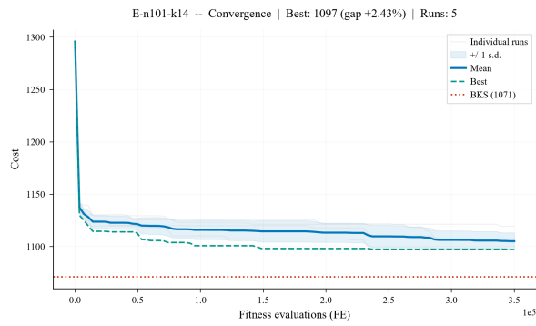
(c) E-n101-k14 (Set E)
