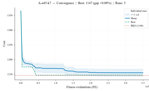
(a) A-n45-k7 (Set A)
