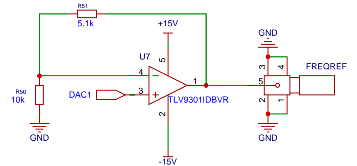
DAC1 OP Amp 0-5V for TTL freq ref for external lock-in
