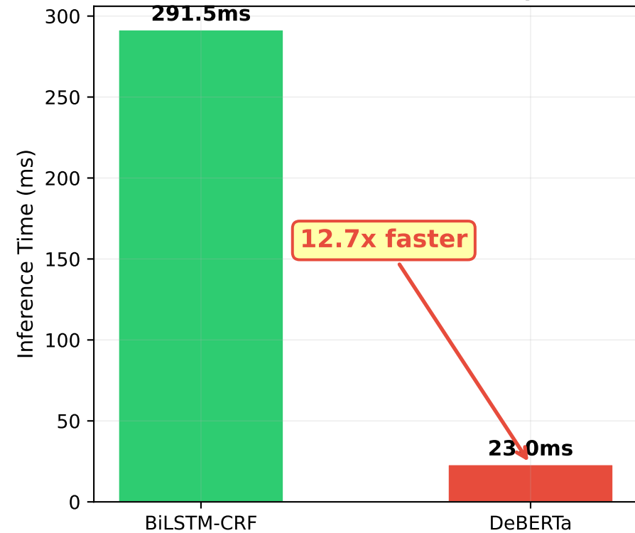
Computational Efficiency
