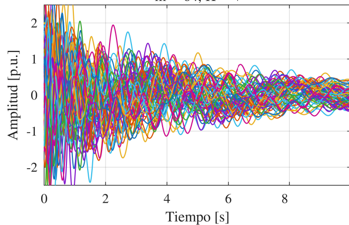
m = 64, K = 4
