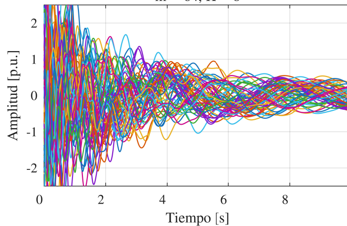
m = 64, K = 8
