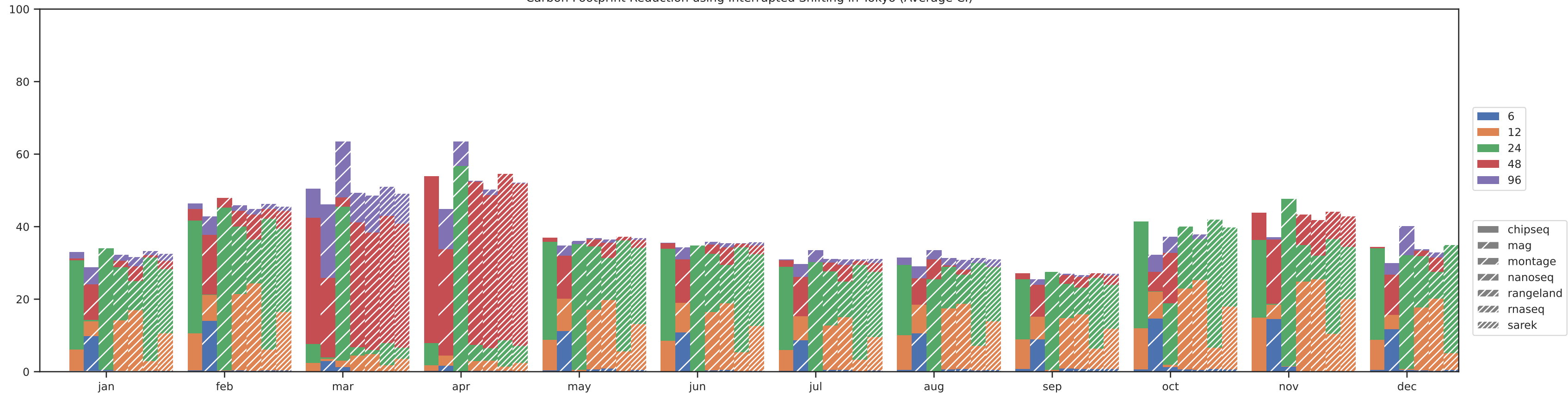
Carbon Footprint Reduction using Interrupted Shifting in Tokyo (Average CI)
