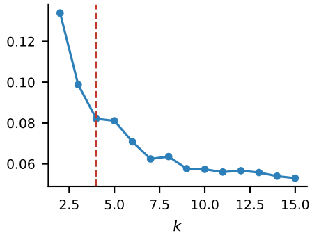
Silhouette \uparrow
