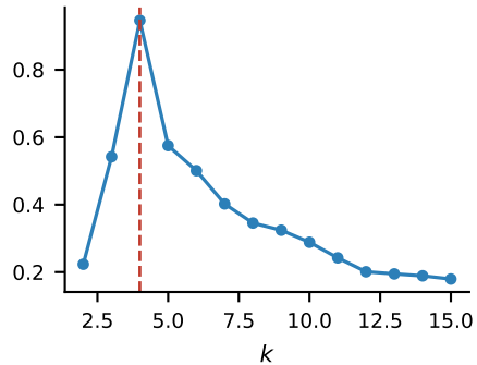
ARI vs. \ published labels
