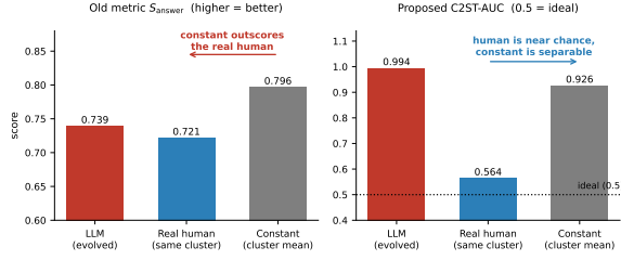
Figure 1: Left: under the old metric the constant outcores a real human. Right: under the proposed C2ST-AUC the human sits near chance (0.5, ideal) and the constant is near-perfectly separable. Only the right panel orders the three correctly.
