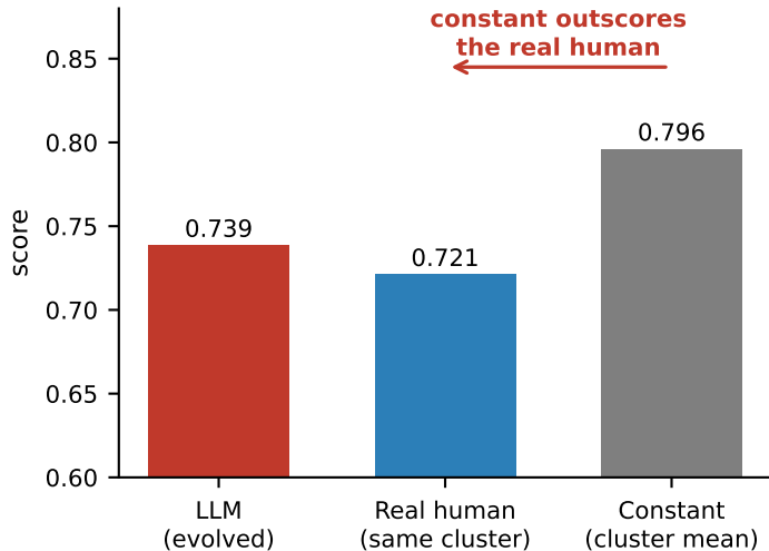
Old metric S_{\text{answer}} (higher = better)
