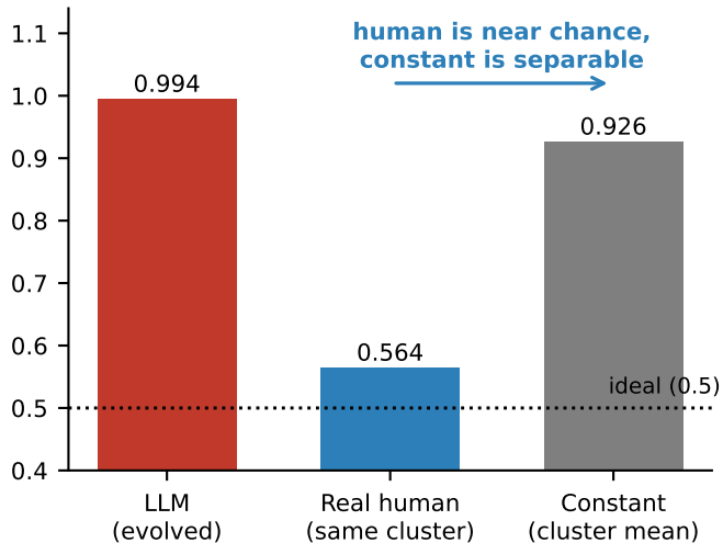
Proposed C2ST-AUC (0.5 = ideal)
