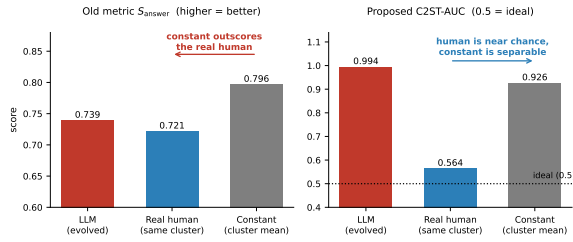
Figure 2: Corrected orientation, 20 cells. Left: under the old metric the constant outscores a real human. Right: under C2ST-AUC (lower is better) the human sits near chance (0.5) while model and constant are both highly separable. Only the right panel places the human above the constant.
