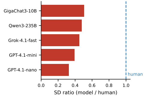
Figure 1: Response spread relative to the humans being simulated, as a ratio of standard deviations. Every model is substantially under-dispersed.
