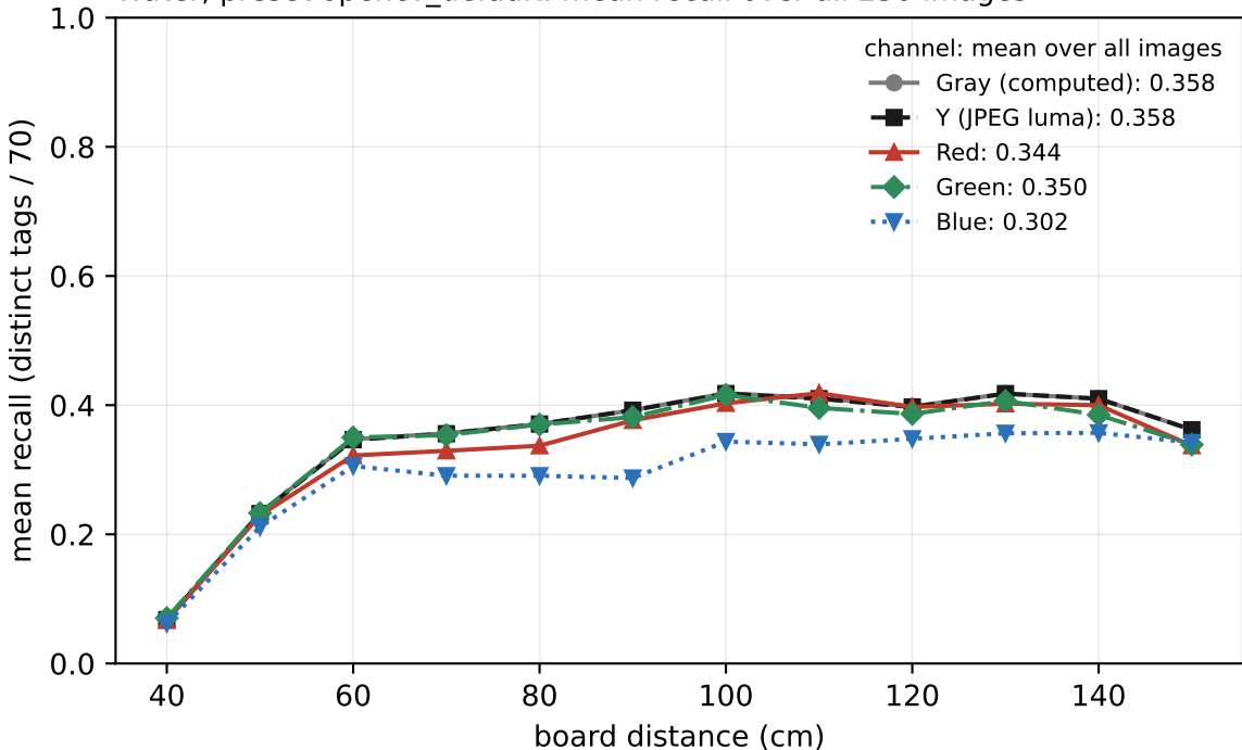
Water, preset opencv_default: mean recall over all 230 images
