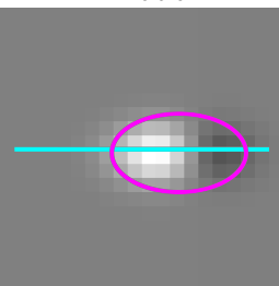
Cell 127 | tau 1.71 Data 0 | Env 0 d 0 FFT 0 d 0
