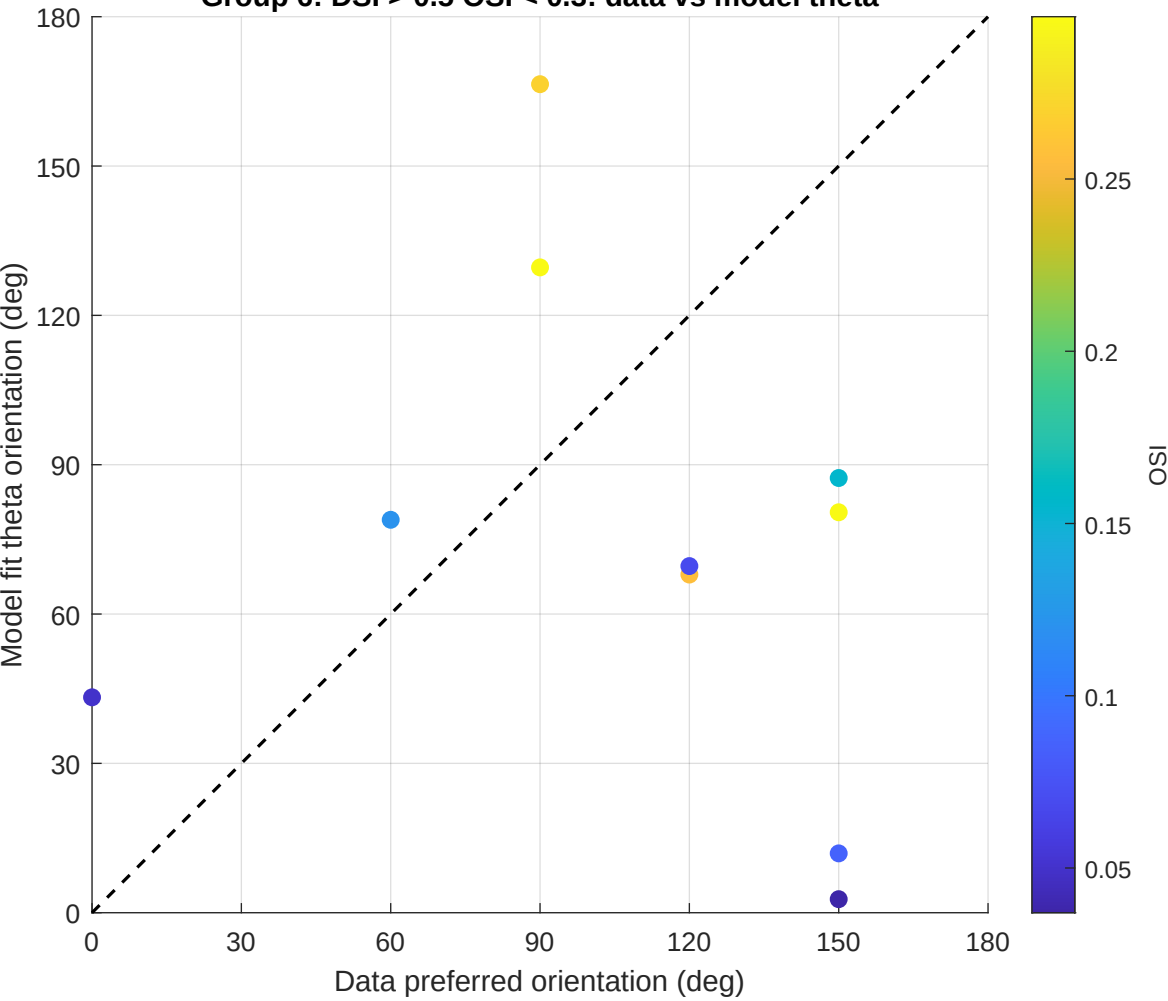
Group 6: DSI > 0.5 OSI < 0.3: data vs model theta
