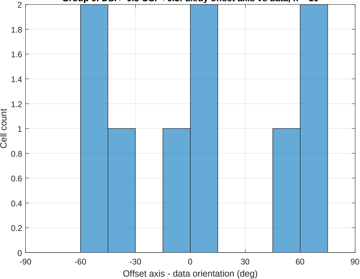
Group 6: DSI > 0.5 OSI < 0.3: dx/dy offset axis vs data, n = 10
