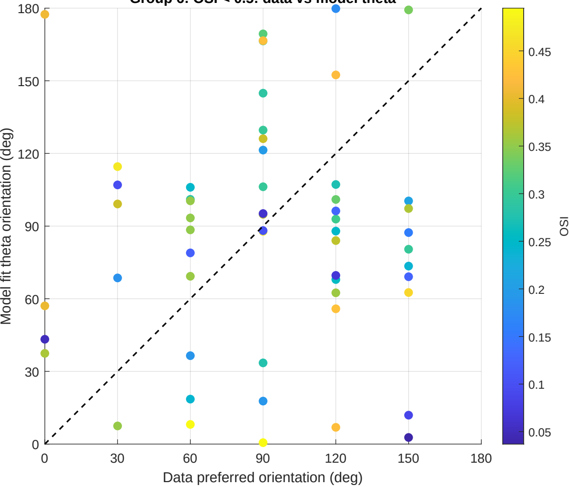
Group 6: OSI < 0.5: data vs model theta
