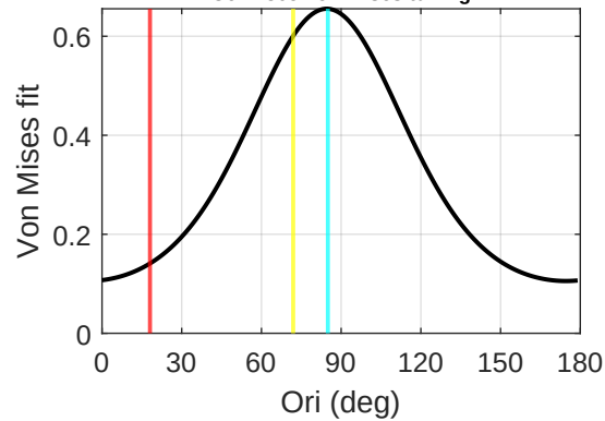
Cell 1865 von Mises tuning
