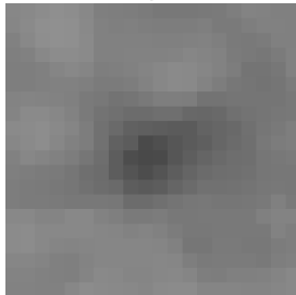
Cell 1822 DSI 0.39 | OSI 0.60
