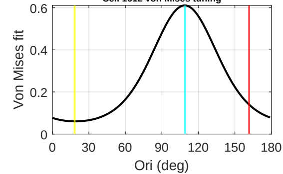
Cell 1612 von Mises tuning
