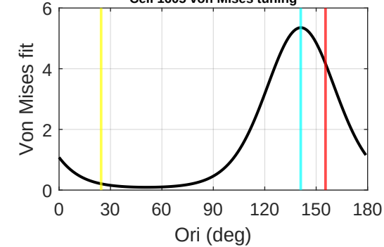
Cell 1605 von Mises tuning
