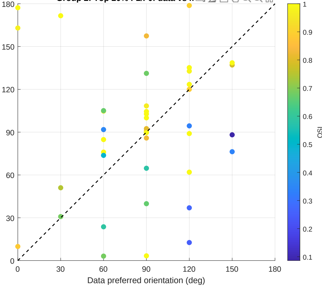
Group 2: Top 20% F1/F0: data vs m
