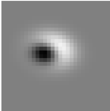
Noncon DoG R^2=0.59 | AICc=-2490.5
