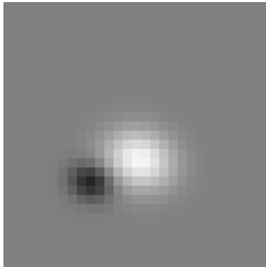
Noncon DoG R^2=0.60 | AICc=-2378.1
