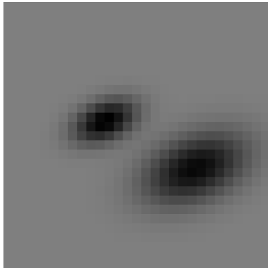
Noncon DoG R^2=0.56 | AICc=-2300.4
