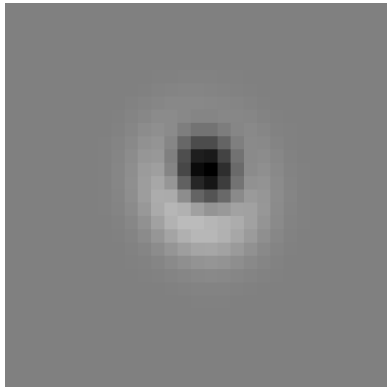
Noncon DoG R^2=0.51 | AICc=-2219.5
